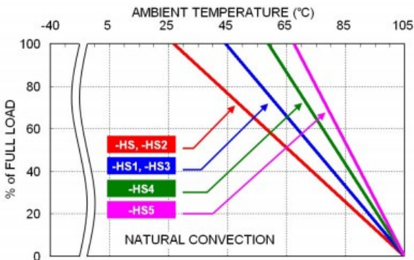
43QAE100-24S05W Derating Curve with Heat-sink (See Thermal Considerations)
