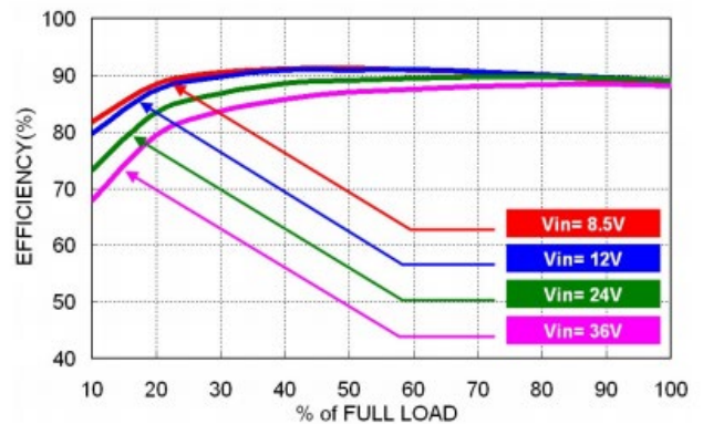
43QAE100-24S05W Efficiency vs. Output Load
