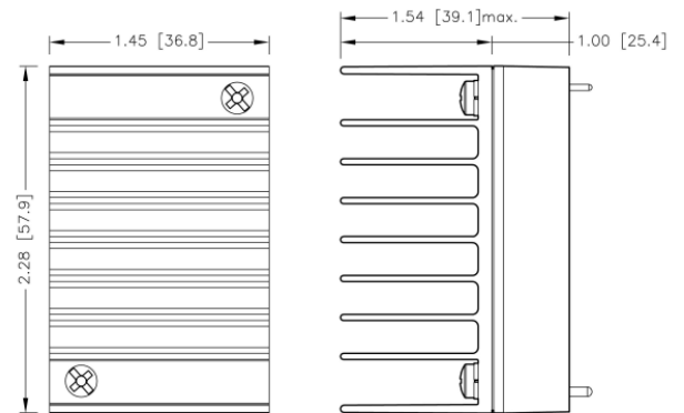
43QAE100-00S00W –HS5 7GA0125P01-F
