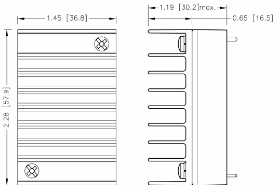
43QAE100-00S00W –HS4 7GA0124P01-F
