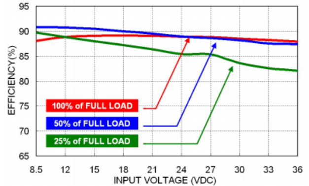
43QAE100-24S05W Efficiency vs. Input Voltage
