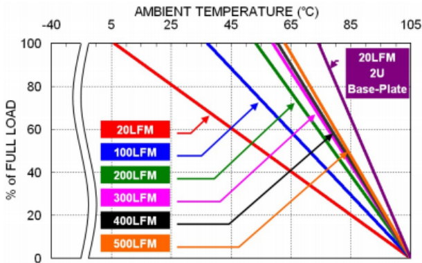
43QAE100-24S05W Derating Curve
